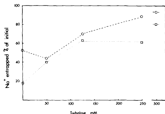
Fig. 1. Retention of ^{22}\text{Na}^+ by dehydrated vesicles as a function of trehalose concentration. Large unilamellar vesicles were dried without prior freezing ( \circ - - - - \circ ), or after freezing in liquid nitrogen ( \square · · · · \square ).
